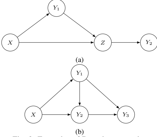
Fig. 2: Examples of Bayesian networks.
